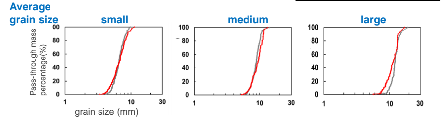
Grain size accumulation curve
